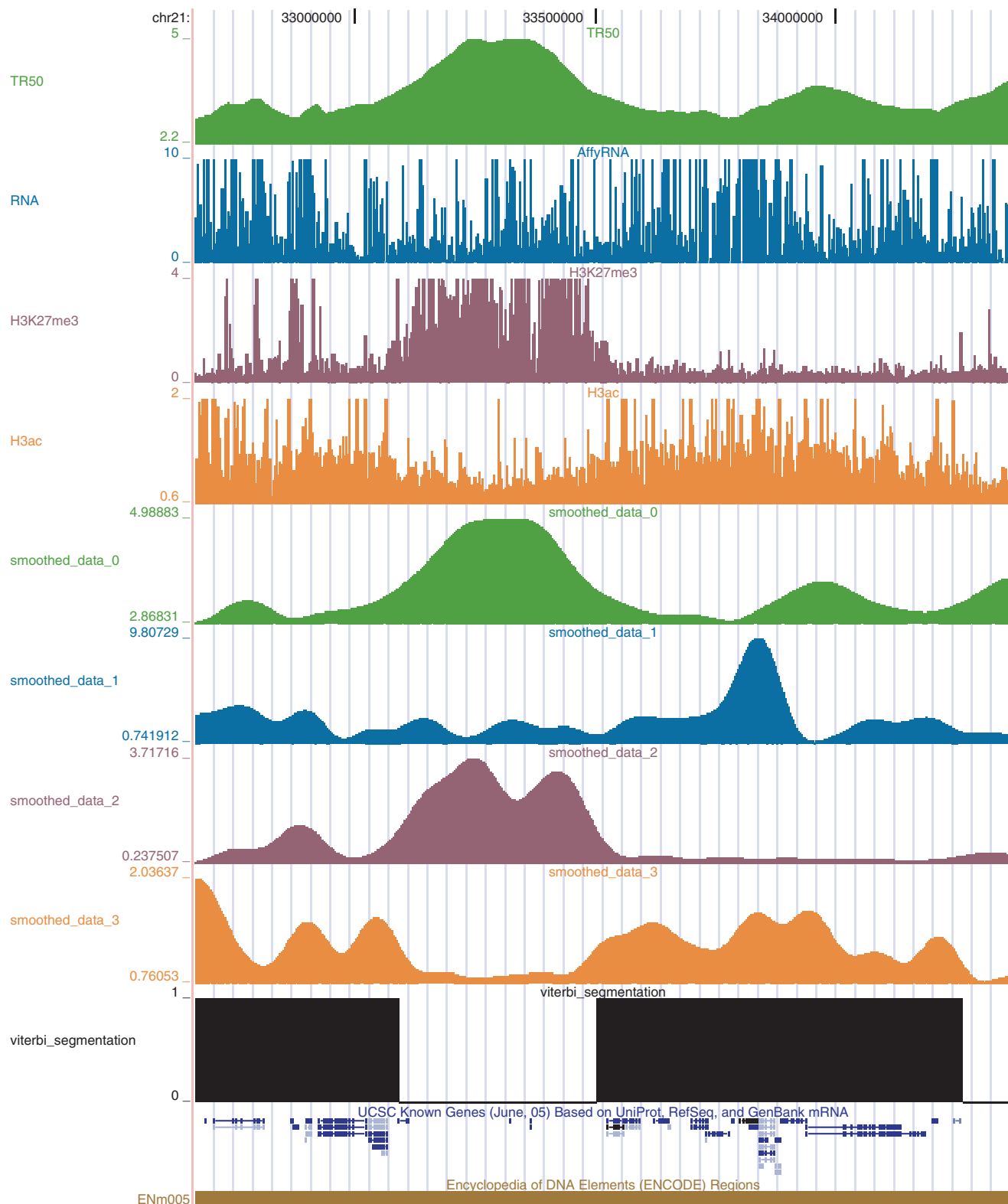
Fig. 2. Multi-datatype functional domains defined using HMMSeg. Shown in this 1.7 Mb region on chr 21 (ENCODE region ENm005) are raw data (top) and 64 kb smoothed data (bottom) for DNA replication timing (green), RNA transcription (blue) and histone modifications H3K27me3 (purple) and H3ac (orange). Row nine shows a two-state Viterbi segmentation based on all four datasets with active domains in black and inactive in white. Note the concentration of genes (bottom row) within active domains. (Data displayed in UCSC Genome Browser with colors added later.)
